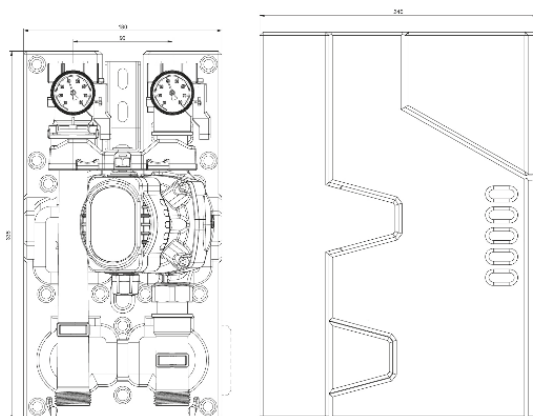
Dimensions (mm)
