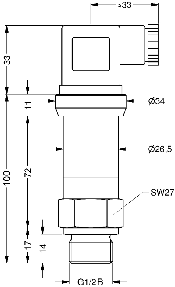
Dimensions (mm)
