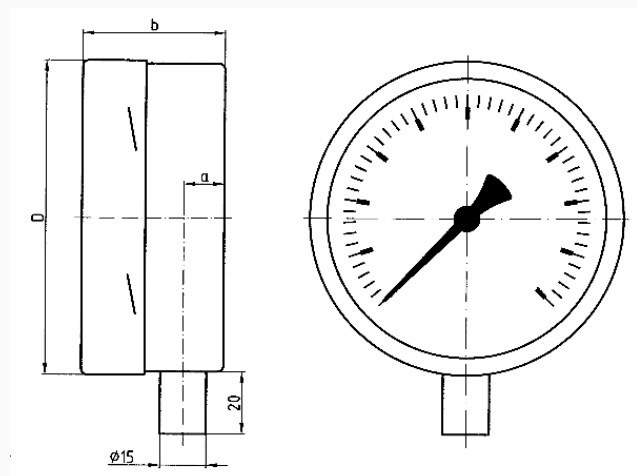
Dimensions (mm)
