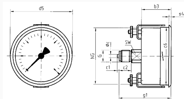
Dimensions (mm)
