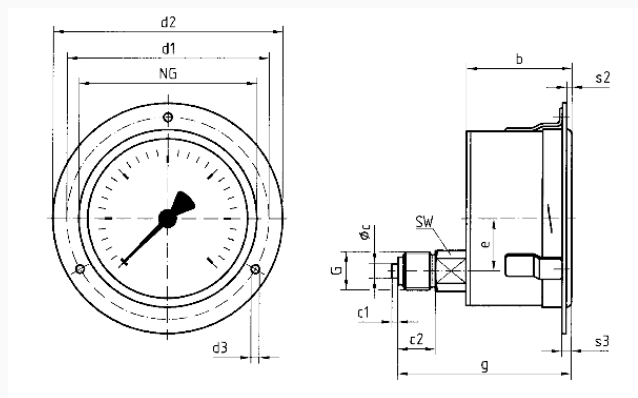
Dimensions (mm)
