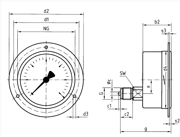
bottom back connection, 3-hole fixing, panel mounting bezel
